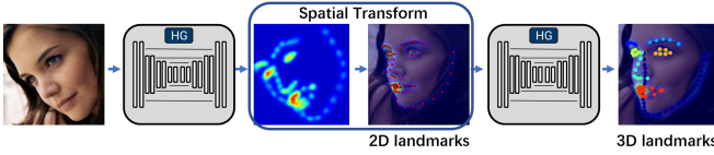
Fig. 4. 2D alignment acts as spatial transform network for 3D alignment.
