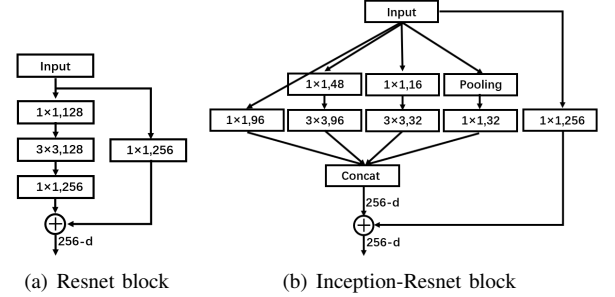
Fig. 2. Resnet and Inception-Resnet blocks to construct Hourglass model.
